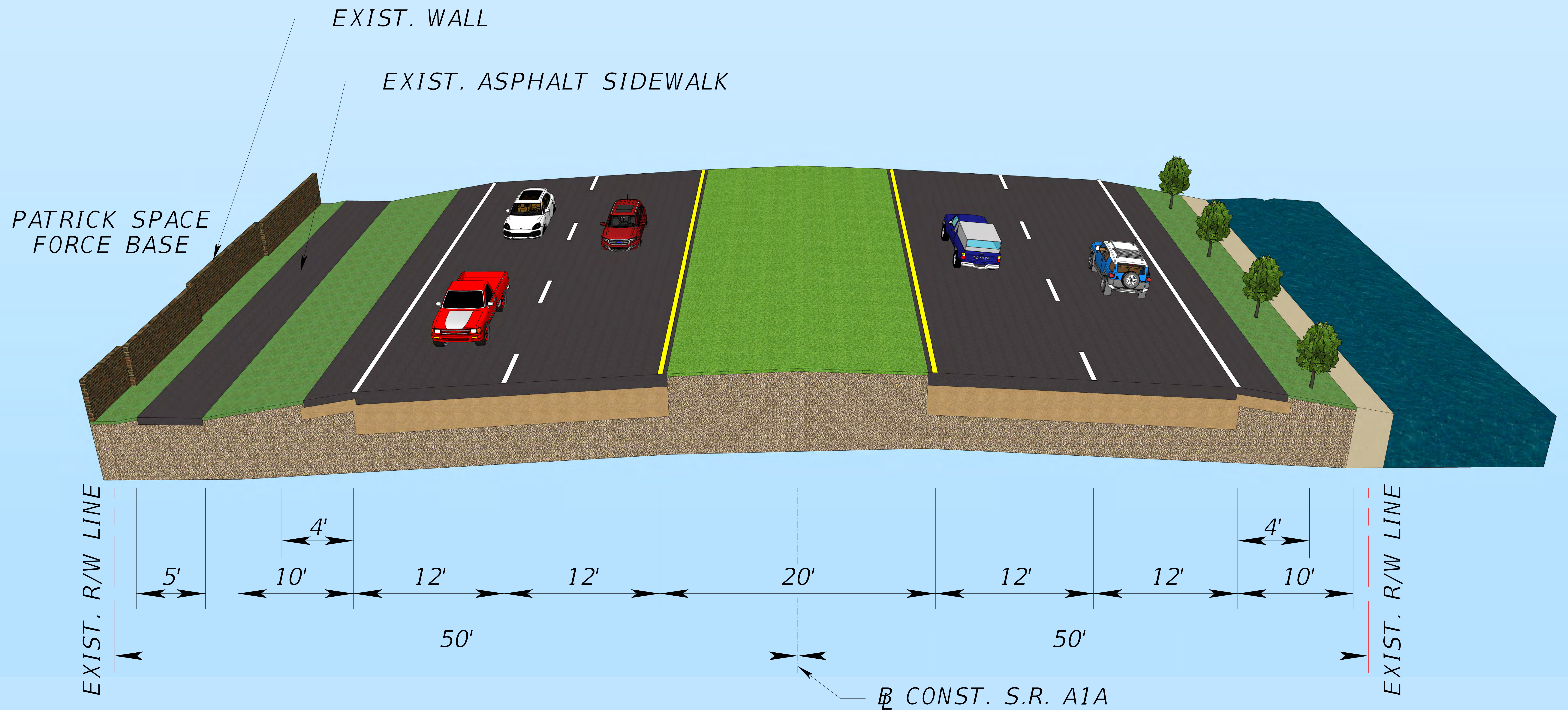
TYPICAL SECTION NO. 2 FROM SOUTH OF SCHOOL AVENUE TO SOUTH OF SHERRY LEE LANE APPROXIMATE SEGMENT LENGTH: 3.2 MILES
