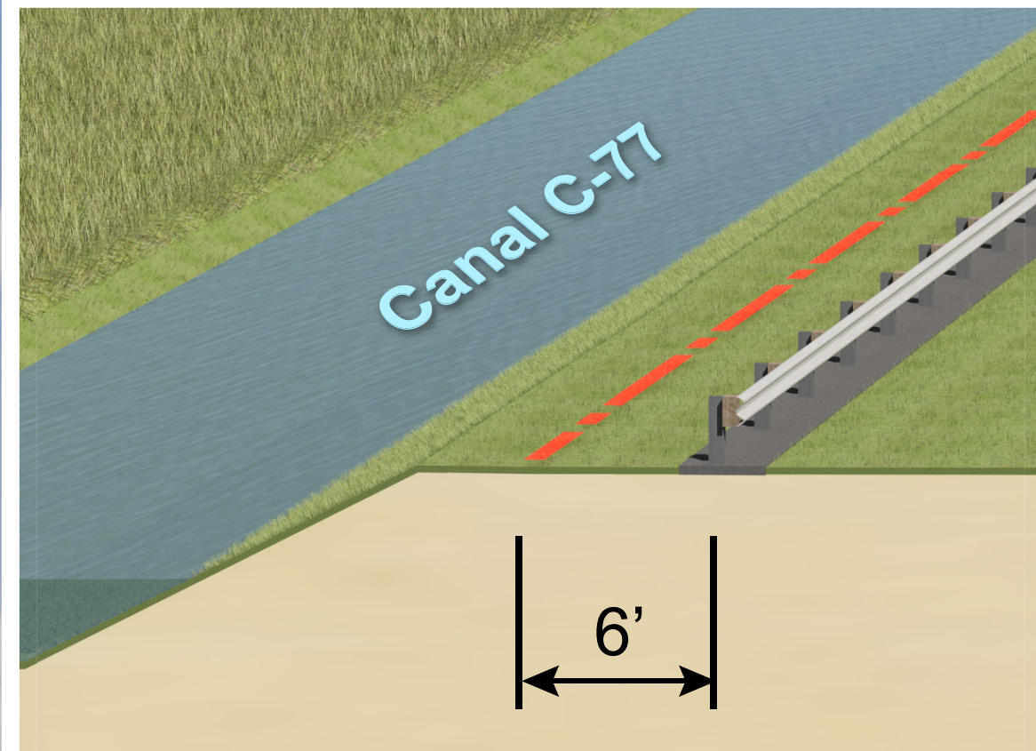
Guardrail Detail
